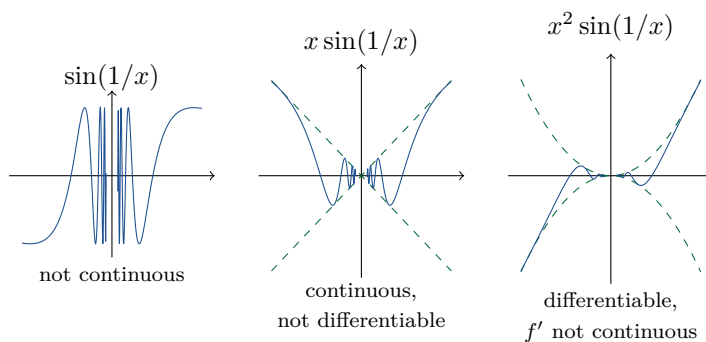
Figure 8.3.1. THREE OSCILLATORY FUNCTIONS. Multiplying by powers of x progressively tames the oscillation of \sin(1/x) near 0.
