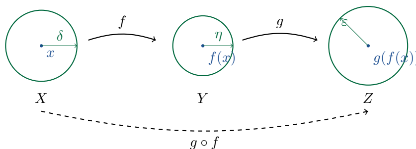
Figure 7.2.5. THE COMPOSITION CHASE. Continuity of g supplies the \eta -ball in Y ; continuity of f supplies the \delta -ball in X whose image lands inside it.
