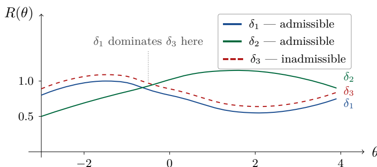
Figure 1.5.13. THREE RISK FUNCTIONS. Risk curves for three decision rules, as sketched in lecture. The dashed rule \delta_3 lies strictly above \delta_1 everywhere, so \delta_1 dominates it and \delta_3 is inadmissible; \delta_1 and \delta_2 cross, so neither dominates the other, and the deck’s legend marks both admissible (1.5.12). A caution when comparing with the deck: its right-edge labels stack \delta_1 above \delta_3 , pairing the names with the wrong endpoints; its legend and its own “ \delta_1 dominates \delta_3 ” annotation—which require the blue curve to be the lower one—are authoritative, and are followed here (edge labels corrected to match the endpoints).
