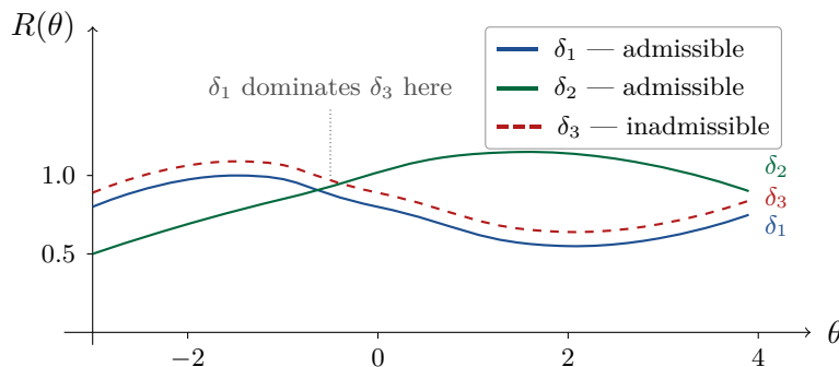
Figure 1.5.7. THREE RISK FUNCTIONS. Risk curves for three decision rules, as sketched in lecture. The dashed rule \delta_3 lies strictly above \delta_1 everywhere, so \delta_1 dominates it and \delta_3 is inadmissible; \delta_1 and \delta_2 cross, so neither dominates the other, and the deck’s legend marks both admissible (1.5.6).
