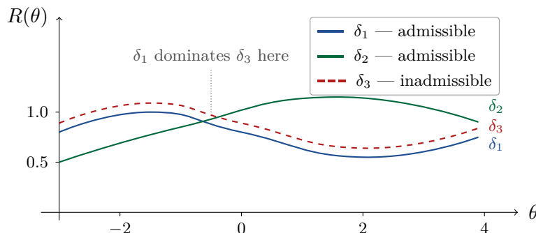
Figure 1.5.14. THREE RISK FUNCTIONS. Risk curves for three decision rules, as sketched in lecture. The dashed rule \delta_3 lies strictly above \delta_1 everywhere, so \delta_1 dominates it and \delta_3 is inadmissible; \delta_1 and \delta_2 cross, so neither dominates the other, and the deck’s legend marks both admissible (1.5.13). A caution when comparing with the deck: its right-edge labels stack \delta_1 above \delta_3 , pairing the names with the wrong endpoints; its legend and its own “ \delta_1 dominates \delta_3 ” annotation—which require the blue curve to be the lower one—are authoritative, and are followed here (edge labels corrected to match the endpoints).
