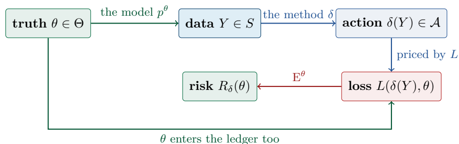
Figure 1.5.11. THE ANATOMY OF A DECISION PROBLEM. How the four objects compose, at one fixed candidate truth \theta : the model hands the data their distribution, the method maps data to an action, the loss prices that action against \theta , and the expectation over the data collapses the randomness to the single number R_\delta(\theta) . Sweeping \theta over \Theta traces the risk curves of Figure 1.5.14 (1.5.1, 1.5.3, 1.5.5, 1.5.9).
