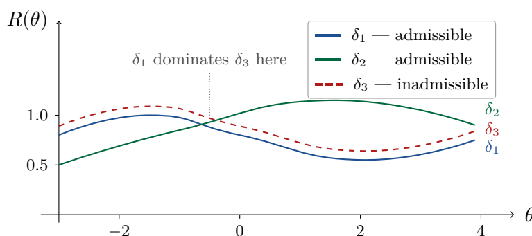
Figure 1.5.7. THREE RISK FUNCTIONS. Risk curves for three decision rules, as sketched in lecture. The dashed rule \delta_3 lies strictly above \delta_1 everywhere, so \delta_1 dominates it and \delta_3 is inadmissible; \delta_1 and \delta_2 cross, so neither dominates the other, and the deck's legend marks both admissible (1.5.6).
