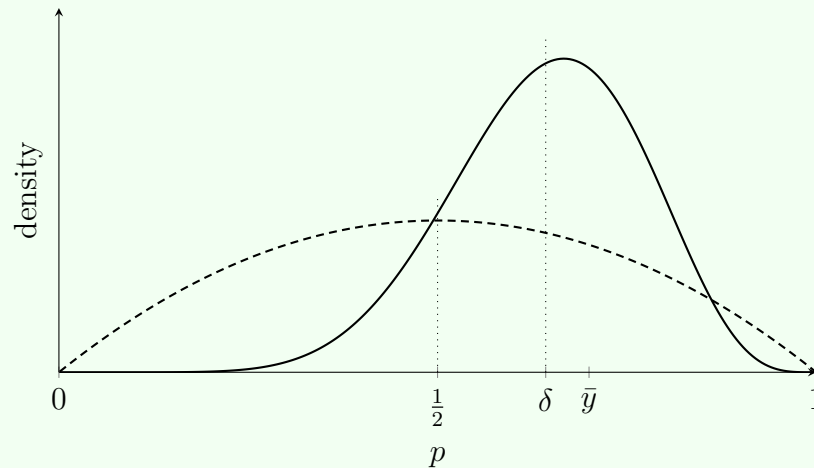
Figure 1. ONE CONJUGATE UPDATE. A Beta(2, 2) prior (dashed, with mean \frac{1}{2} marked) meets n = 10 Bernoulli trials with s = 7 successes and becomes the Beta(9, 5) posterior (solid). The Bayes estimate \delta = \frac{9}{14} \approx 0.643 sits between the prior mean and the sample rate \bar{y} = 0.7 , closer to the data because n outweighs \alpha + \beta = 4 .
