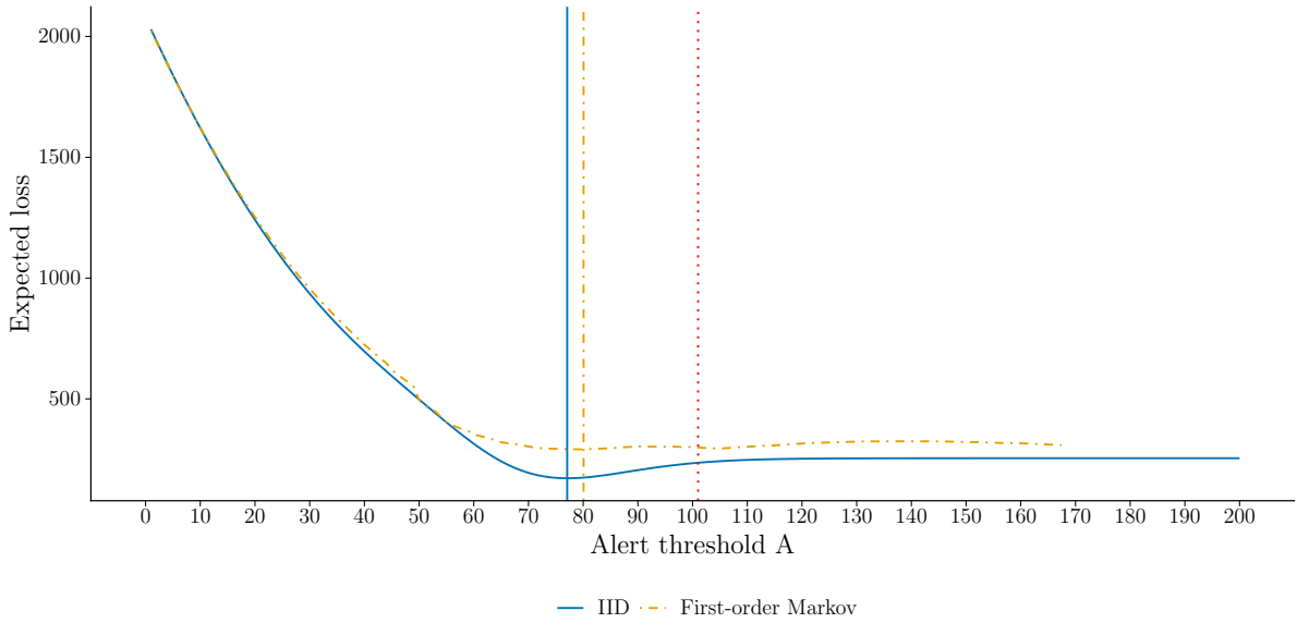
Figure 15: Baseline Expected Loss Curves
