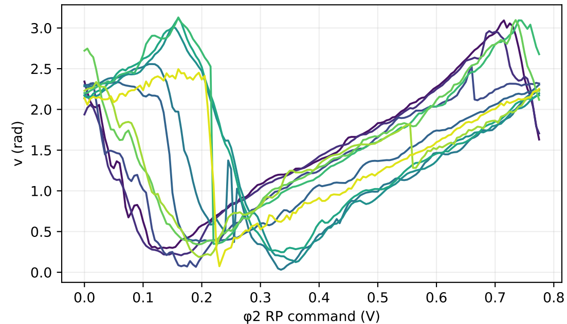
Polar response
