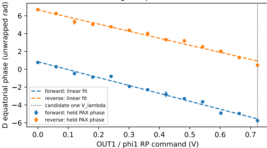
Held-step equatorial means
