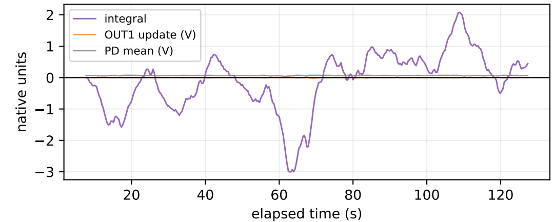
PI state, command increment, and PD
