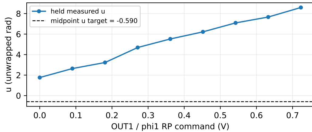
Fresh one-V \lambda u calibration
