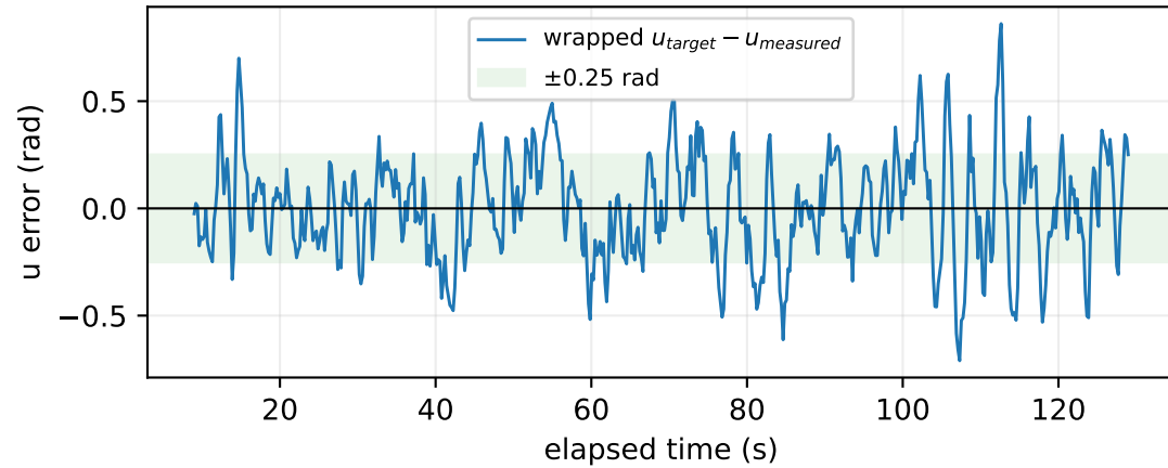
Azimuth locking error
