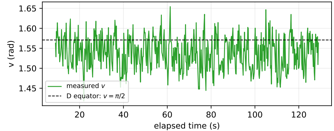
Uncontrolled polar coordinate
