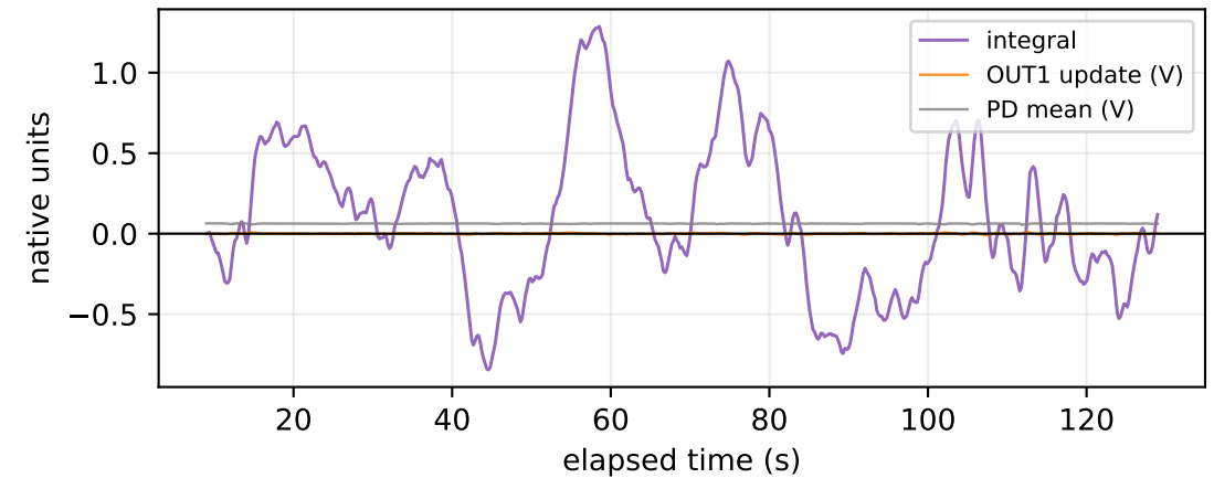
PI state, command increment, and PD
