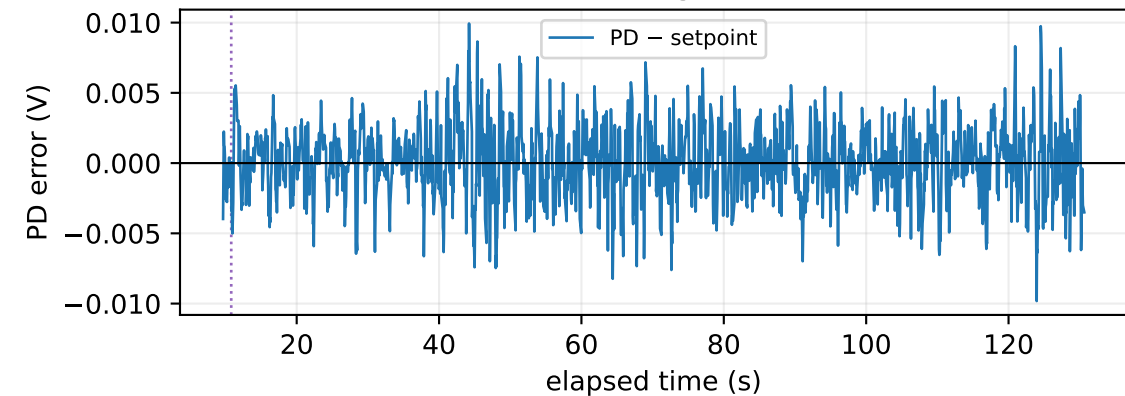
PD locking error
