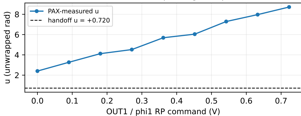
PAX-assisted \phi 1 rough map
