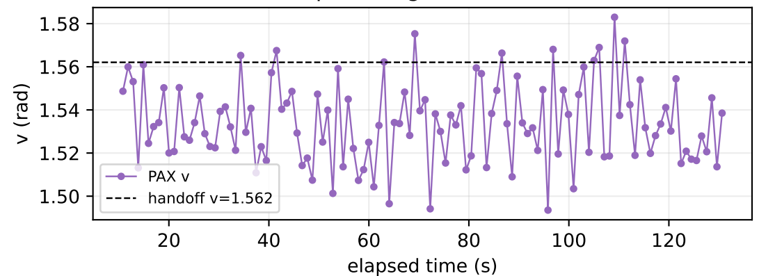
PAX polar-angle cross-check
