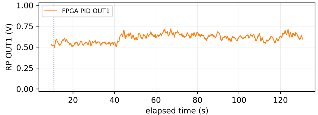
Continuous FPGA actuator output
