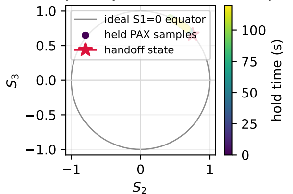
Held lock trajectory on the Poincare equator
