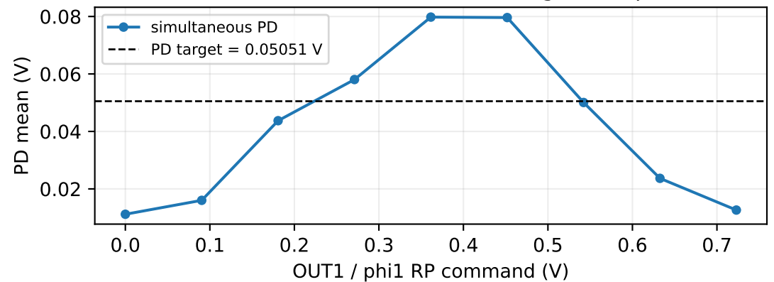
PD value associated with rough u map
