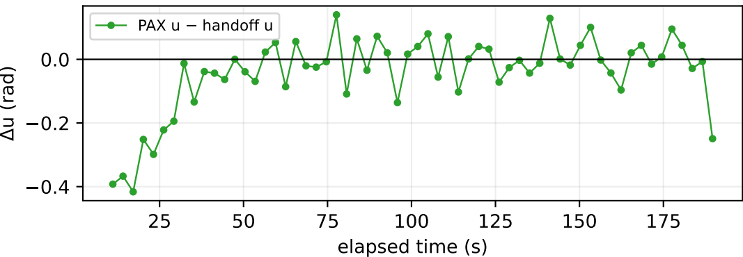
Held lock trajectory on the Poincare equator
