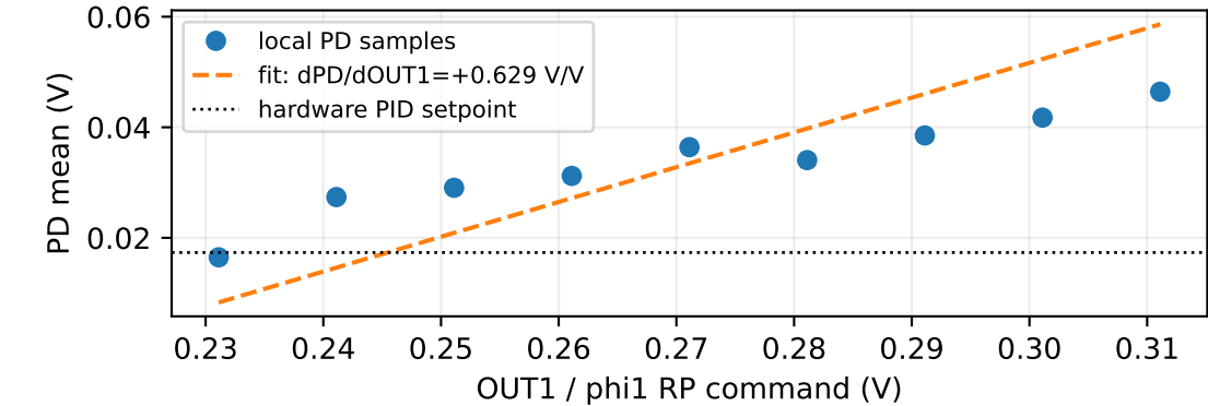
PD locking error
