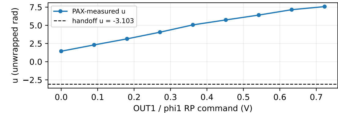
Automatic local PD calibration
