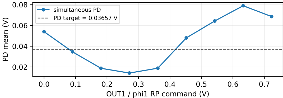
FPGA PD lock
