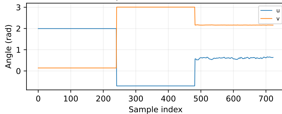
Sphere coordinates
