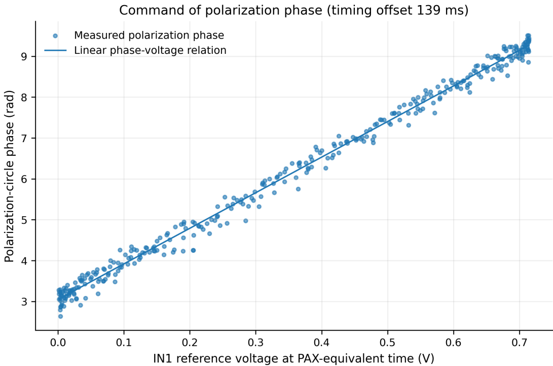
Polarization phase vs command
