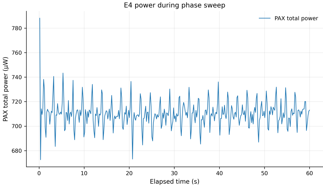
Power during phase sweep
