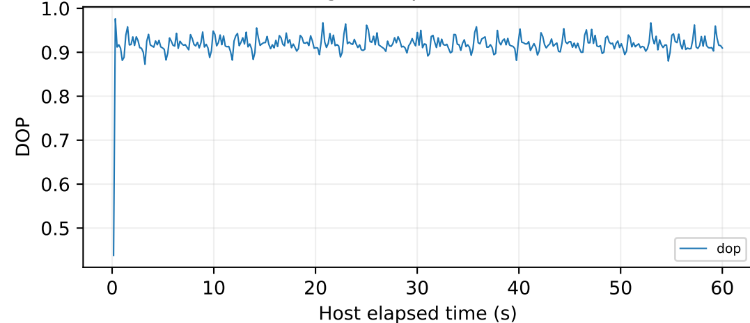
Total-power-normalized Stokes
