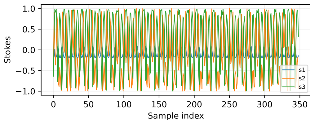
Normalized Stokes
