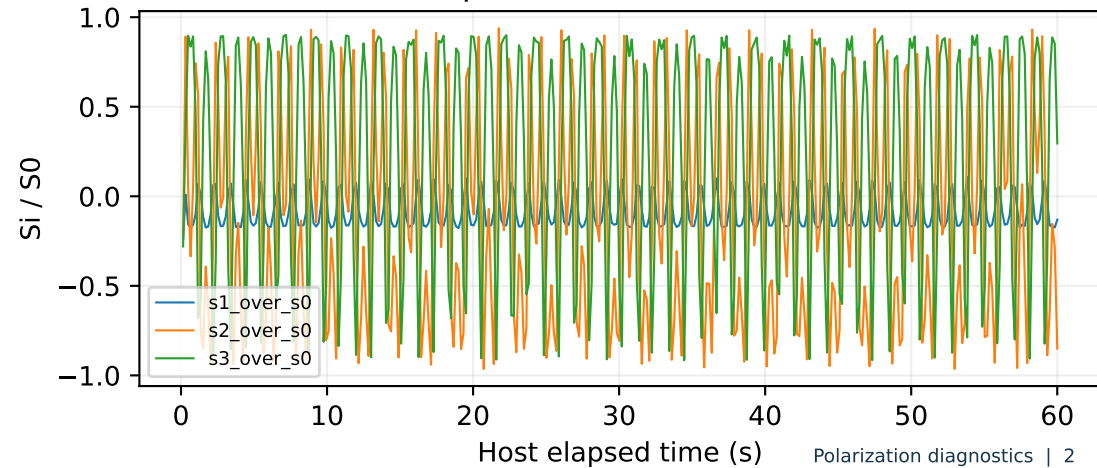
Total-power-normalized Stokes
