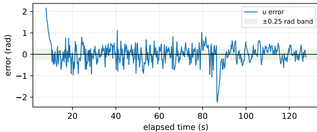
Controlled-coordinate error
