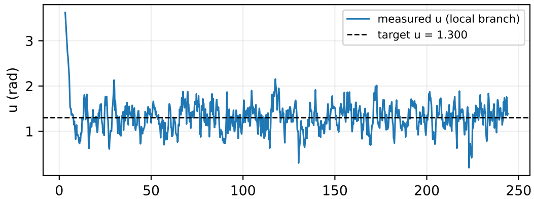
Azimuthal coordinate
