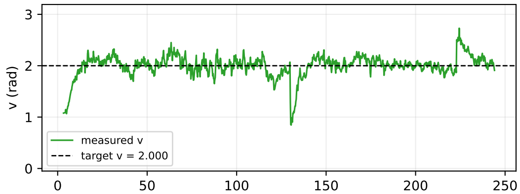
Polar coordinate
