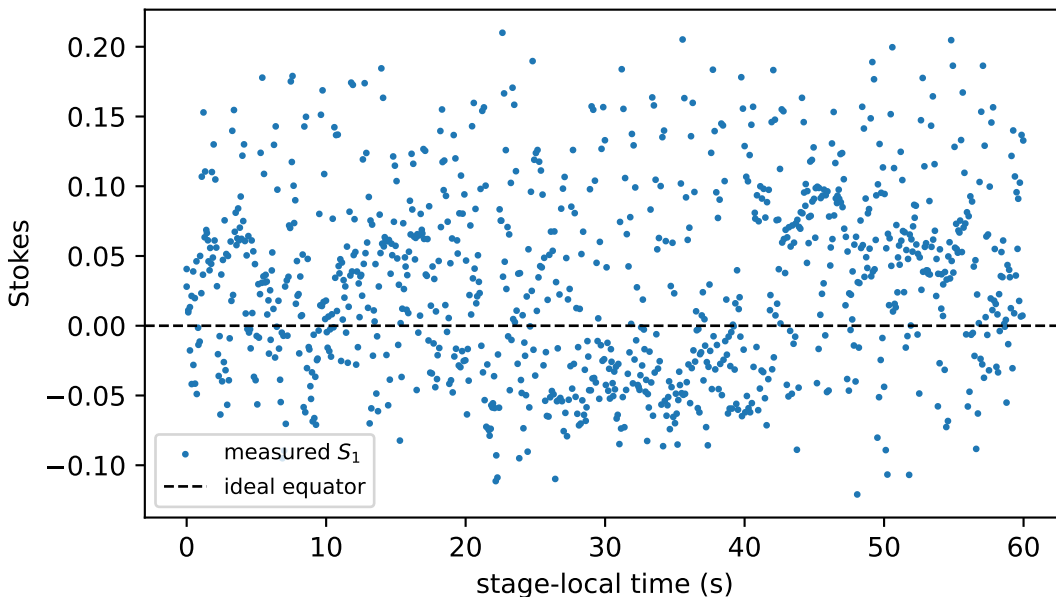
Command-to-polarization transfer
