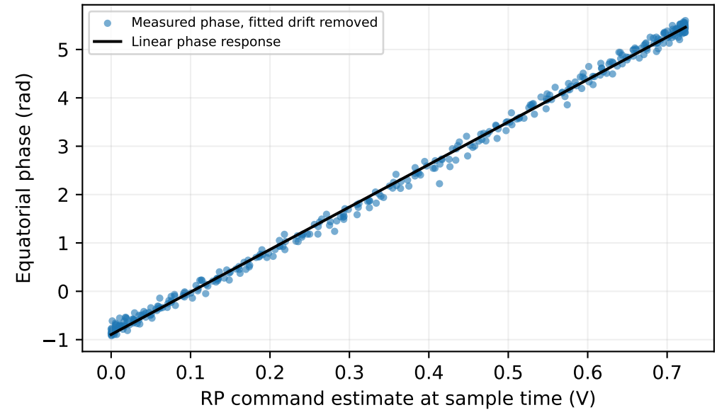
Voltage-to-phase relation (reconstructed command)
