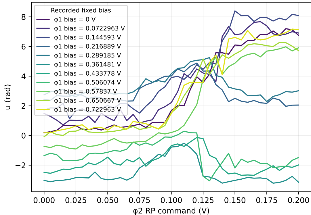
Azimuthal response (unwrapped)
