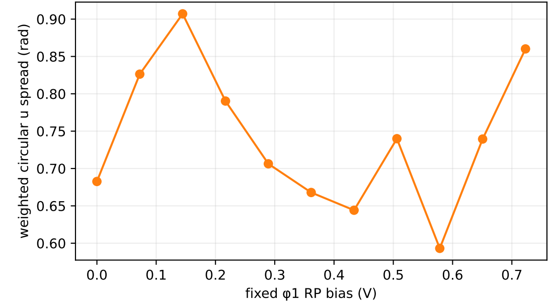
Off-axis azimuth spread (poles downweighted)
