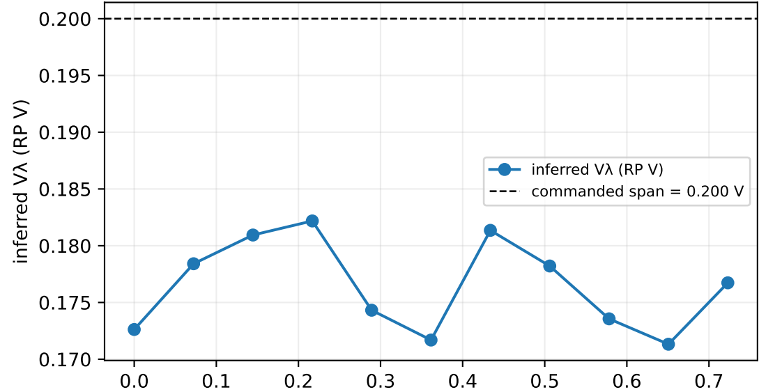
Principal-axis V\lambda versus fixed-axis bias
