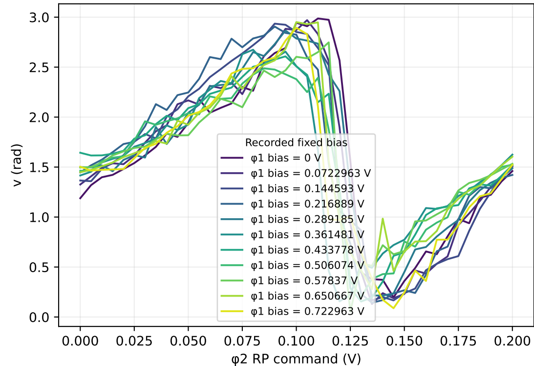
Polar response
