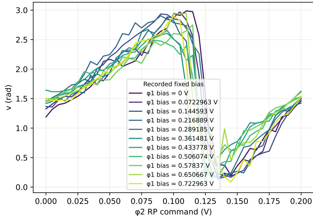
Polar response
