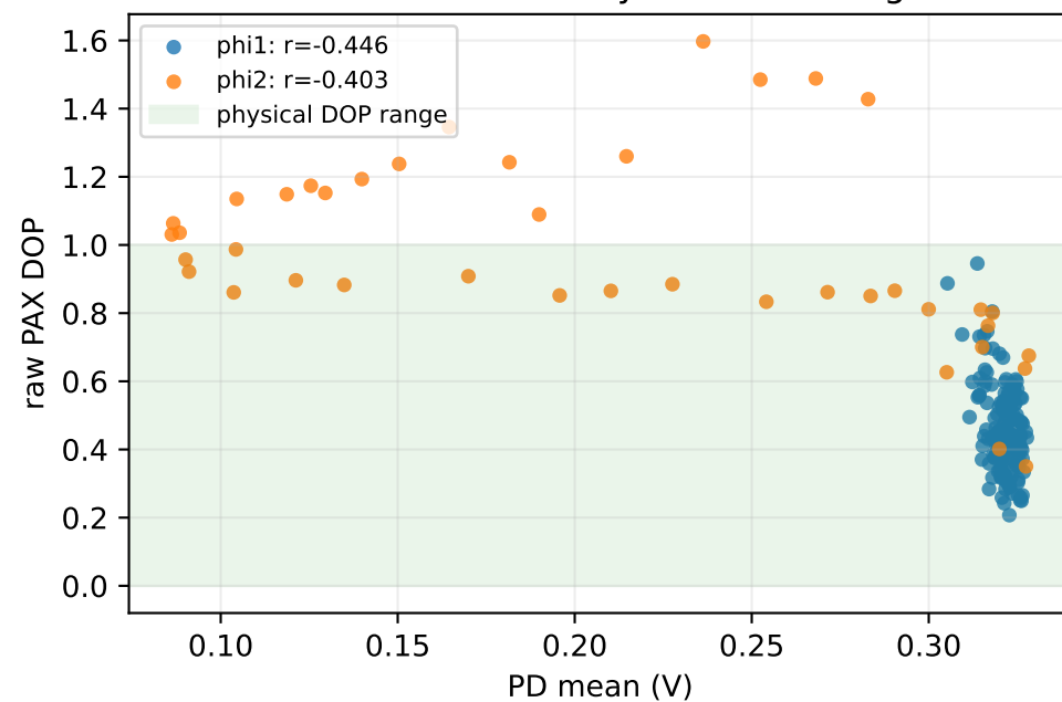
Does raw DOP covary with PD voltage?
