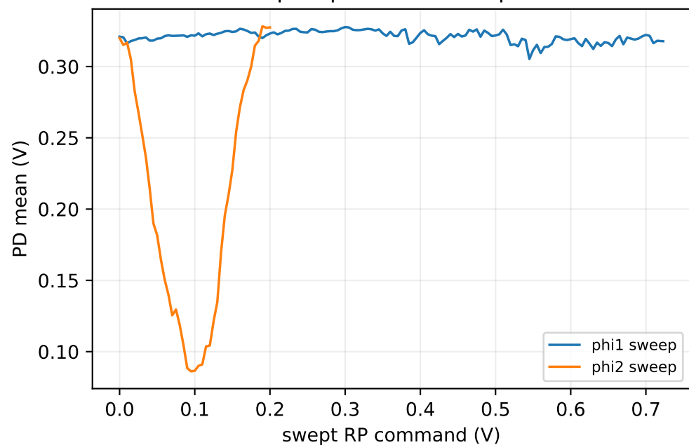
Final-port photodiode response
