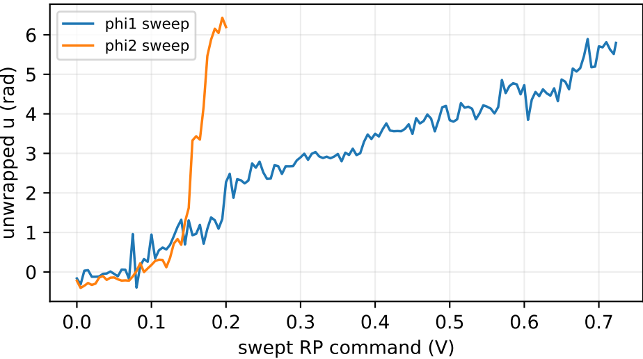
Azimuth response
