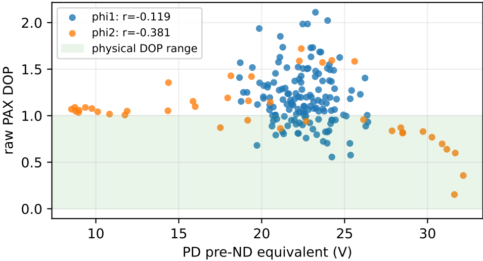
Does raw DOP covary with PD power?
