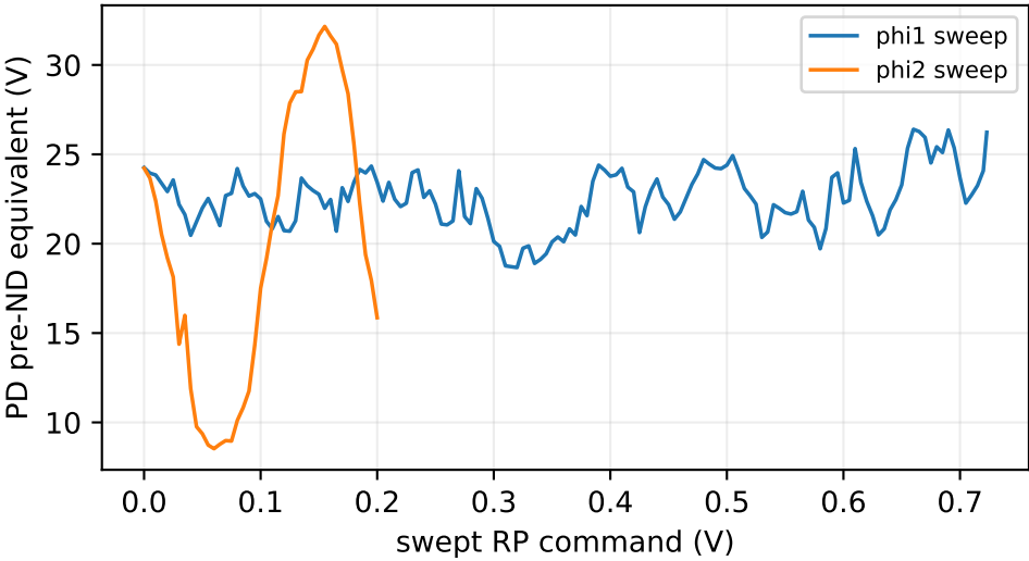
Final-port PD response (corrected for OD 2)
