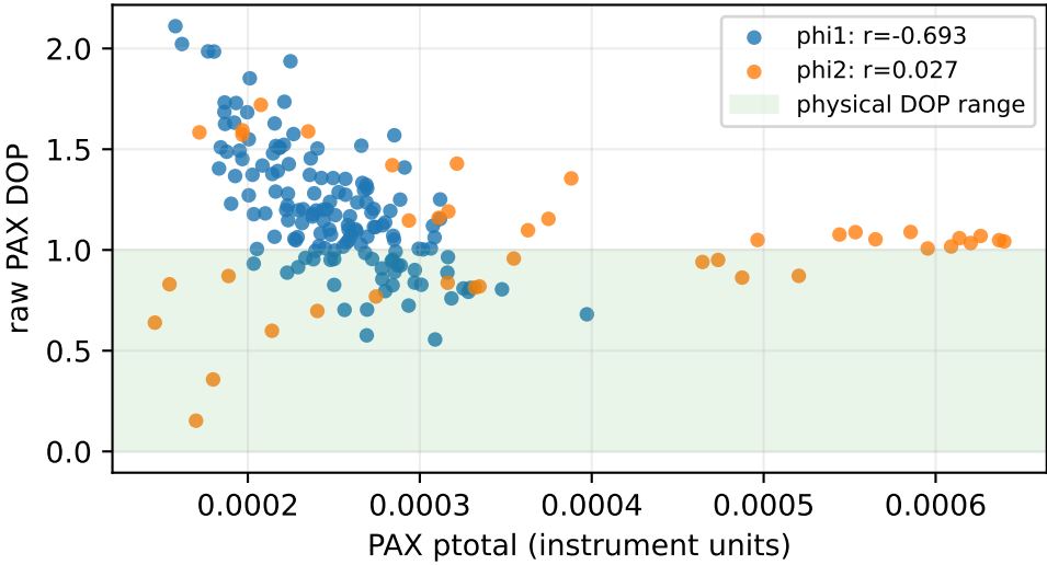
Does raw DOP covary with PAX-port power?
