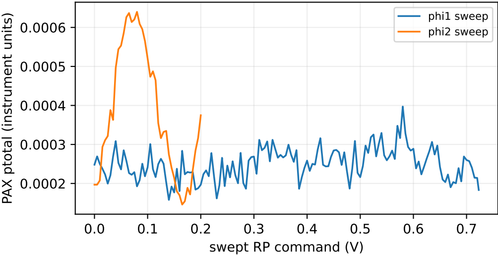
PAX-port total-power response
