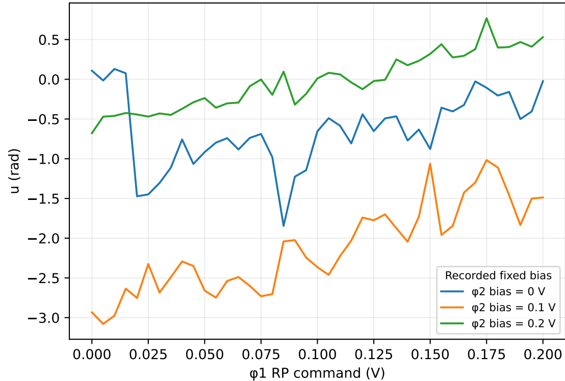
Azimuthal response (unwrapped)
