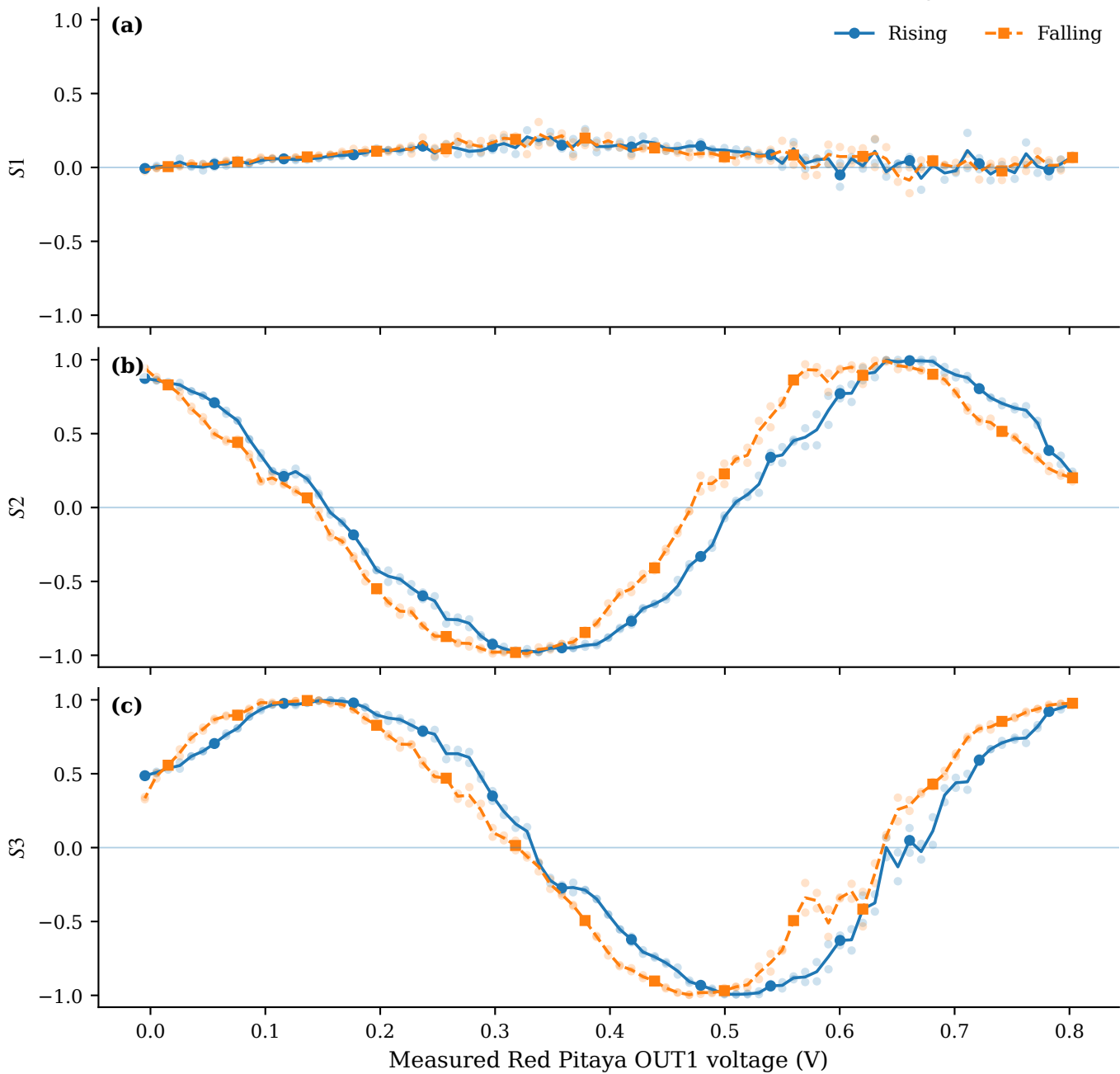
Static polarization transfer versus measured drive voltage
