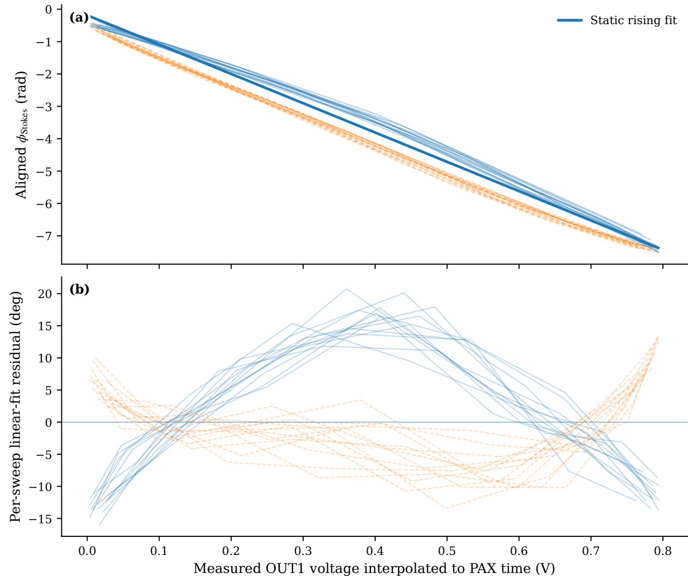
Dynamic polarization-transfer repeatability (measured electrical frequency 0.4657 Hz)
