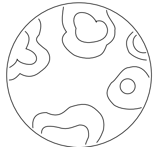
fcPlanetD
