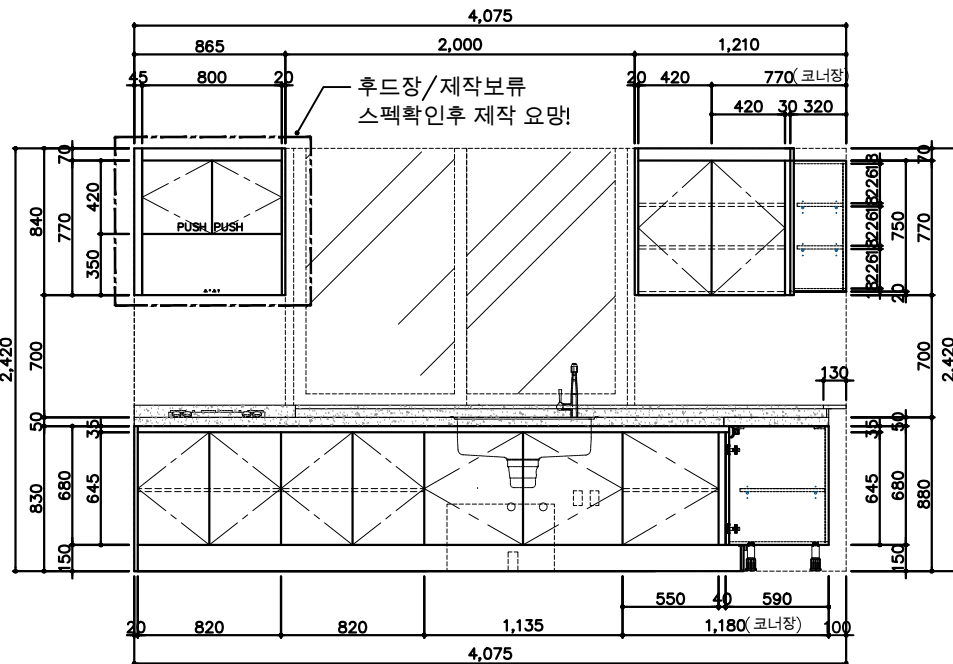
FRONT VIEW - A
