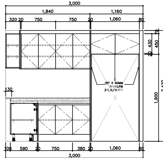
FRONT VIEW - B
