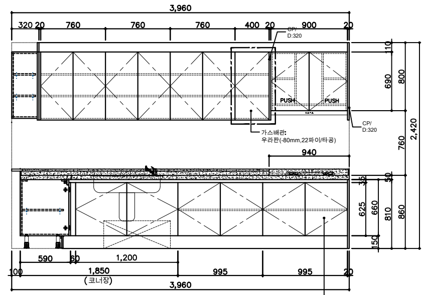
FRONT VIEW - B
