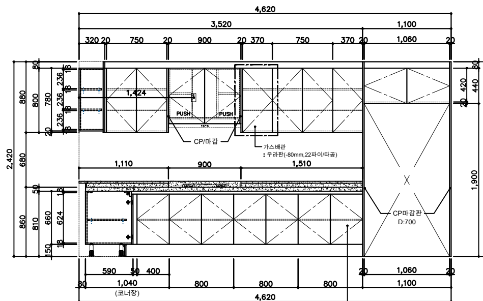
FRONT VIEW-B
