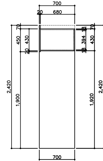
SIDE VIEW - B
