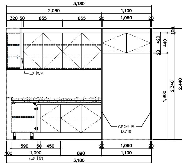
FRONT VIEW-B
