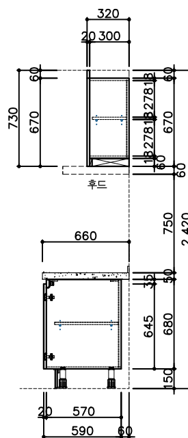
SIDE VIEW - A
