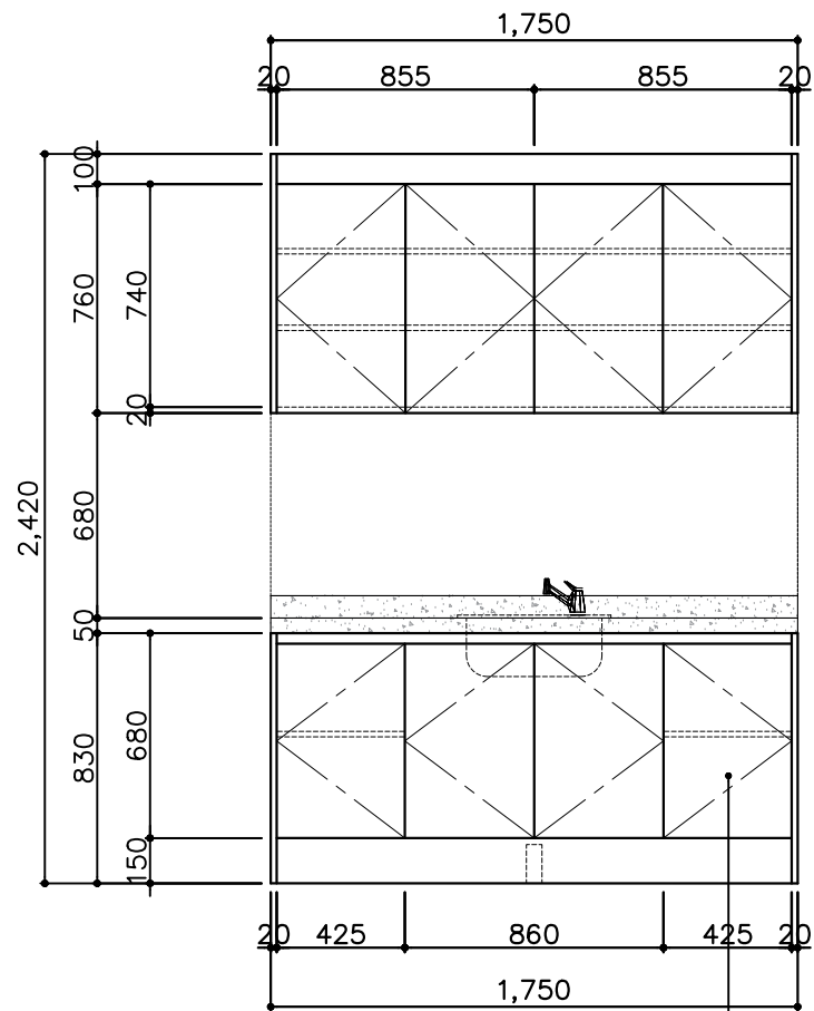
FRONT VIEW
