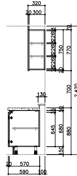
SIDE VIEW - B
