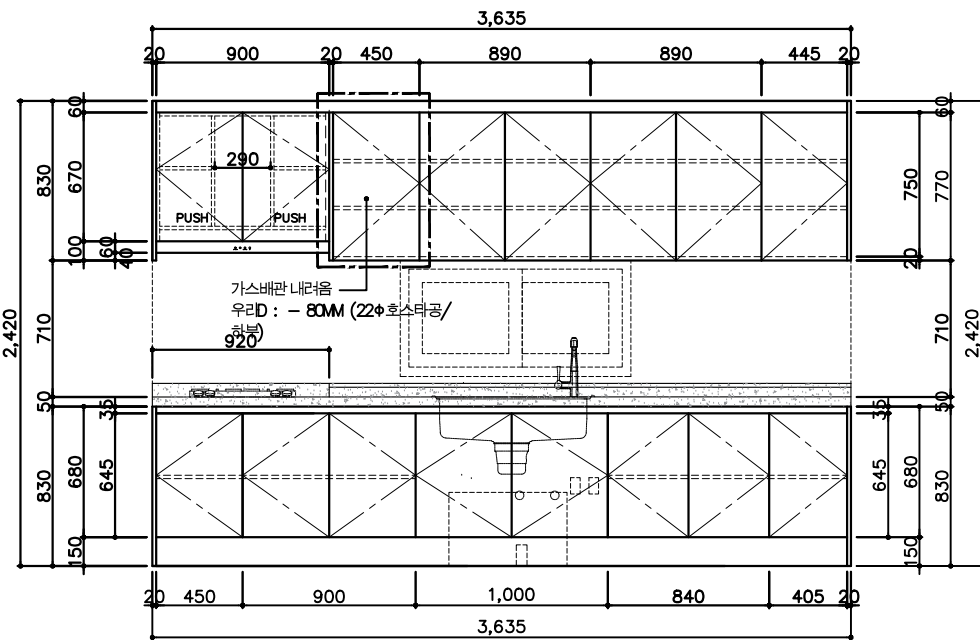
FRONT VIEW - A
