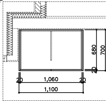
TOP VIEW - B
