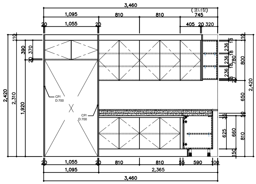
FRONT VIEW - A
