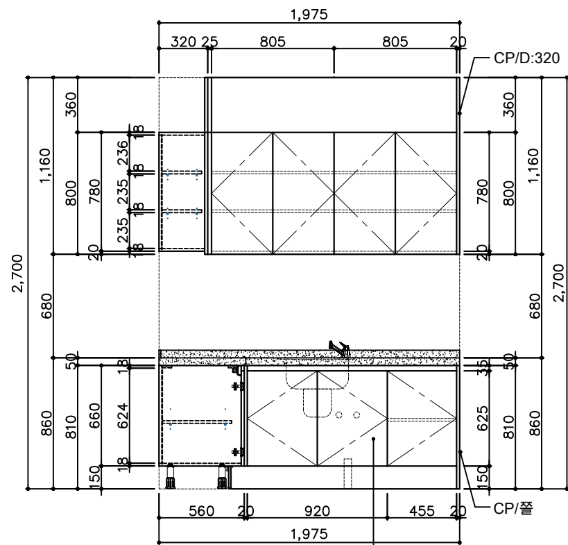
FRONT VIEW-A
