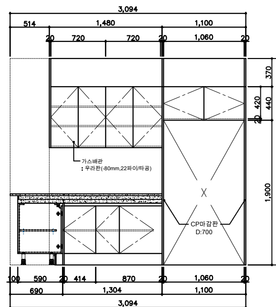
FRONT VIEW-B
