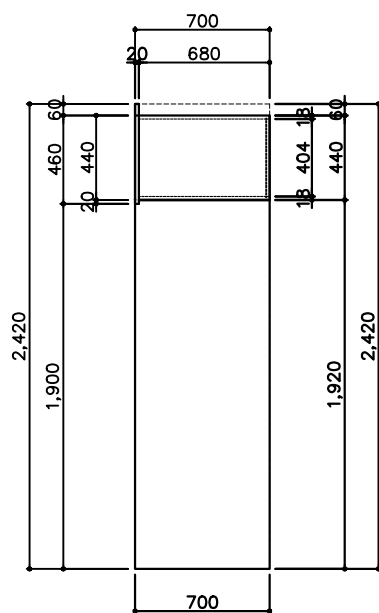
SIDE VIEW - B
