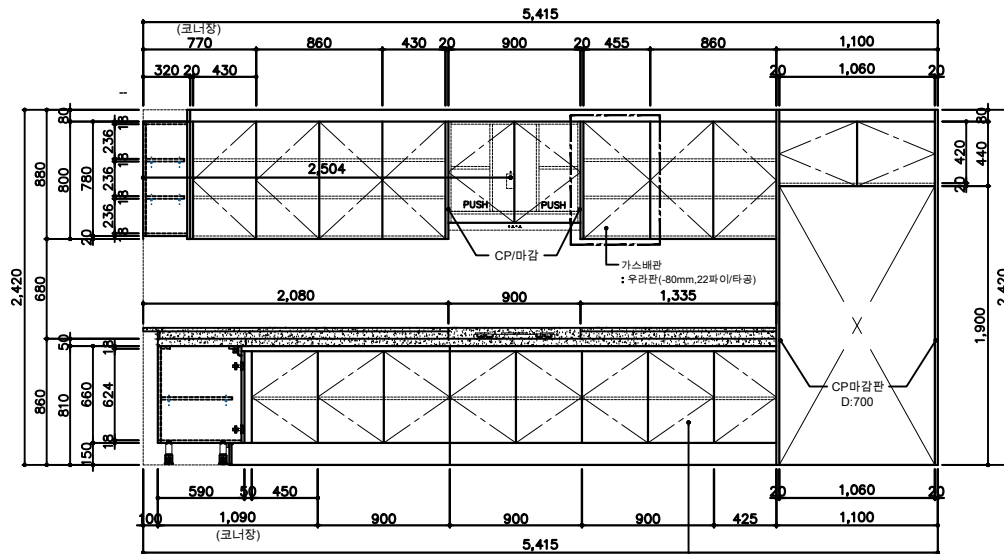
FRONT VIEW-B
