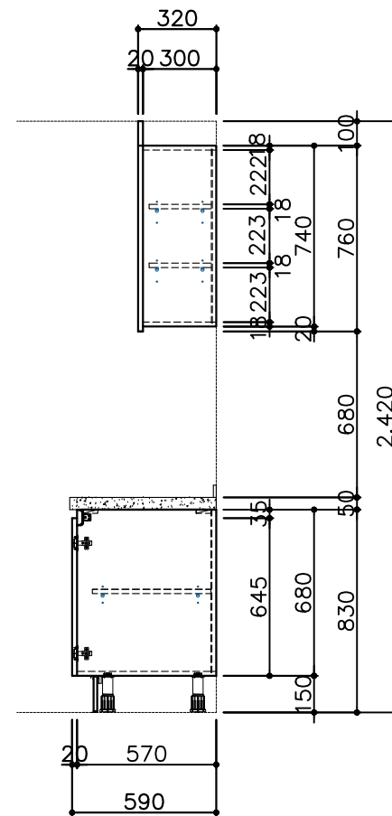
SIDE VIEW
