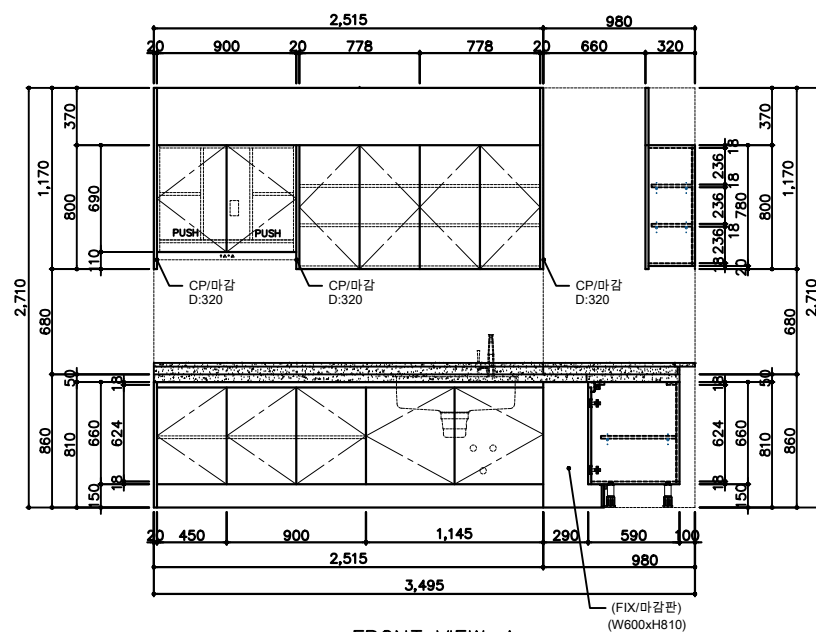
FRONT VIEW-A
