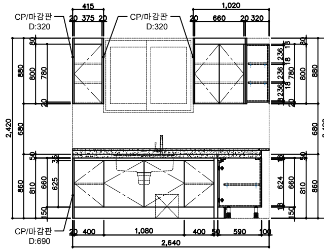
FRONT VIEW-A
