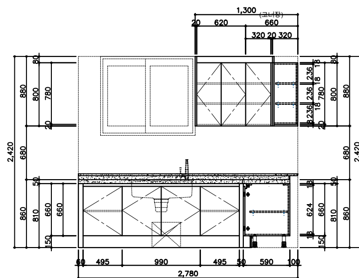
FRONT VIEW—A
