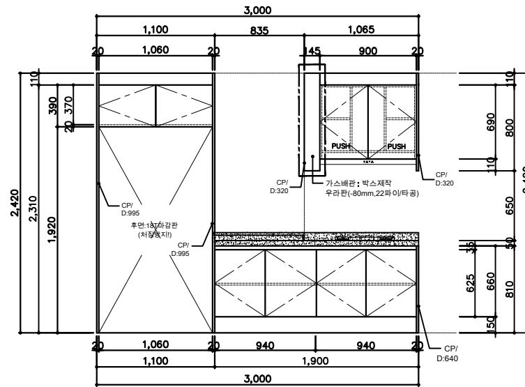
FRONT VIEW - B
