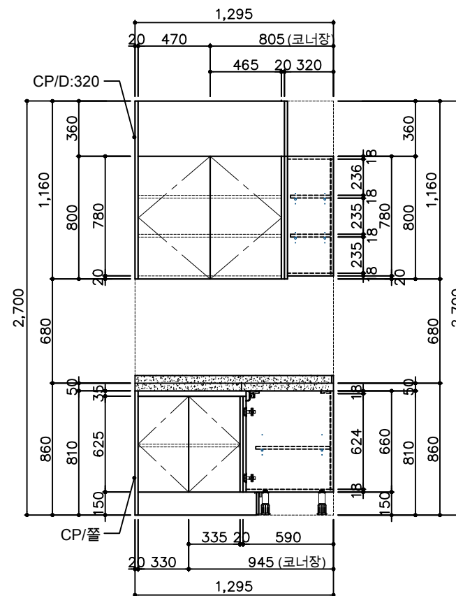
FRONT VIEW-B
