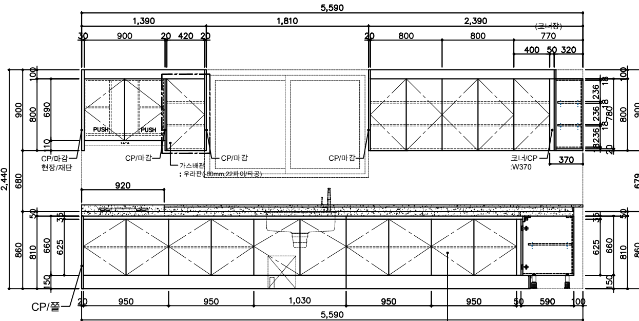
FRONT VIEW-A
