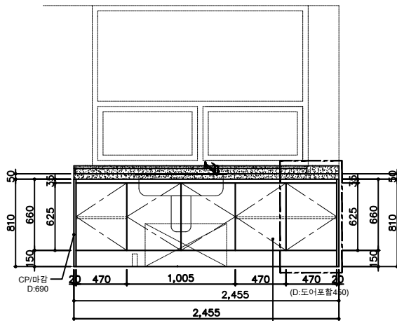
FRONT VIEW - A
