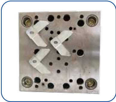
风阀角码连续模具 Air Valve Duct Corner
