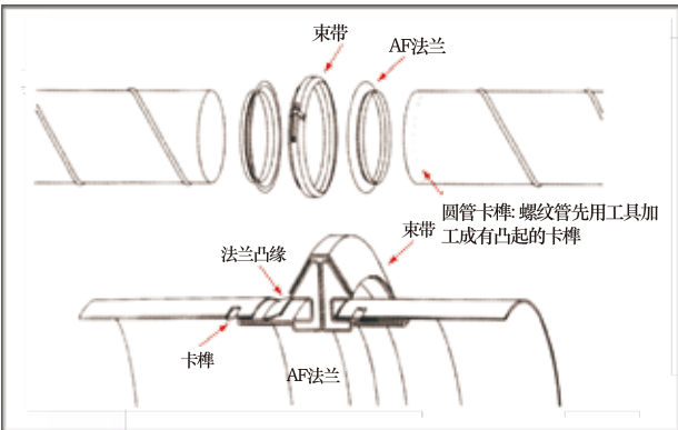
芯管连接 Core connect
