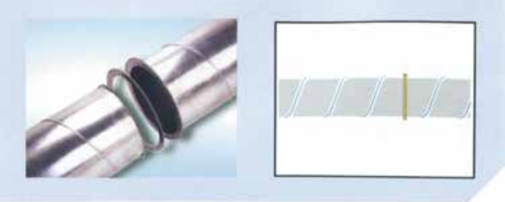
扁钢法兰连接 Flat steel flange connect
