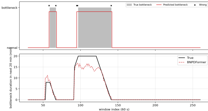
next-window bottleneck state
