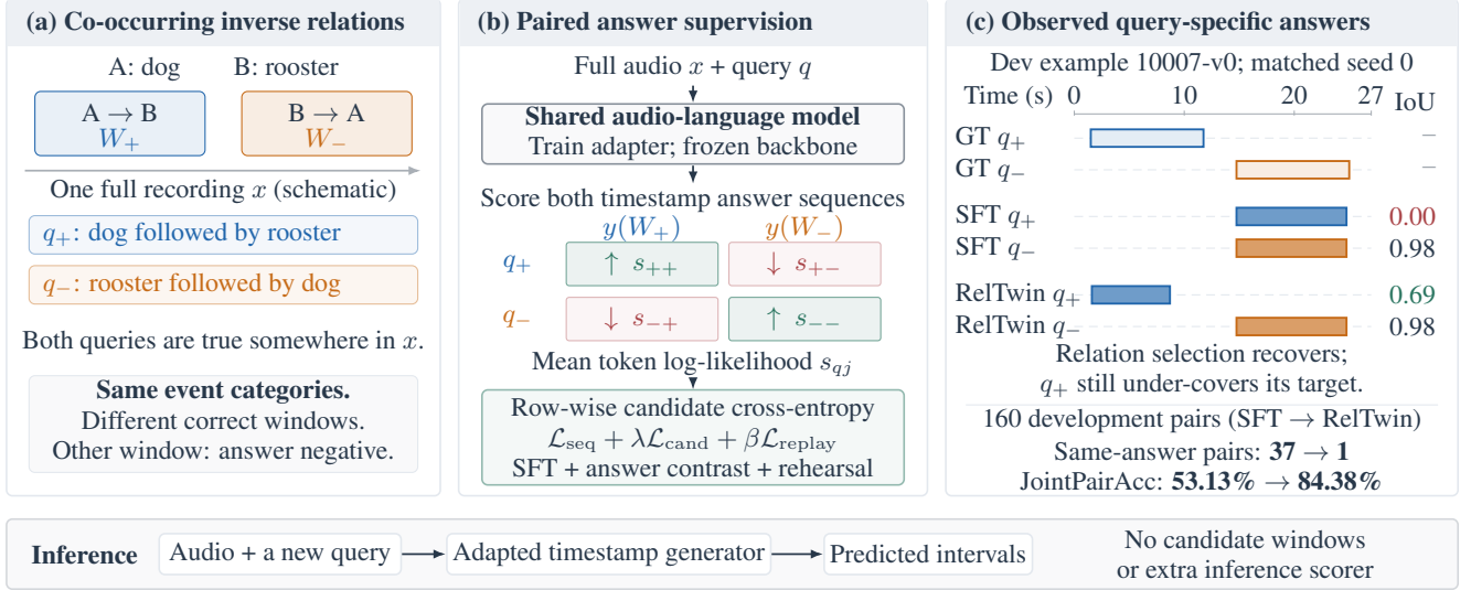
Fig. 1. RelTwin overview. (a) Co-occurring inverse relations supply locally confusable answers. (b) The shared model contrasts timestamp sequences during training; arrows denote target preferences. (c) A cached seed-0 example (queries 56–57) shows relation recovery and boundary under-coverage. Aggregate statistics cover all 160 development pairs. The bottom path shows candidate-free timestamp generation at inference.
