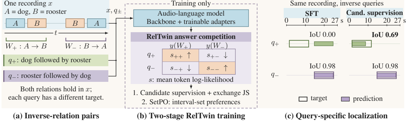
Fig. 1. RelTwin binds inverse queries to different windows in one recording. (a) Reused excerpts form two local targets. (b) Candidate supervision and exchange consistency precede SetPO; diagonal cells mark correct answers and arrows indicate preferences. (c) In the SpotSound-A mechanism experiment, candidate supervision recovers query-specific windows from SFT’s repeated answer. Outlines mark targets; filled bars show predictions, evaluated by set-IoU.
