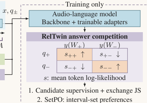
(b) Two-stage RelTwin training
