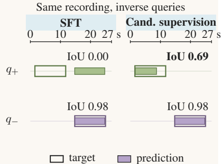
(c) Query-specific localization
