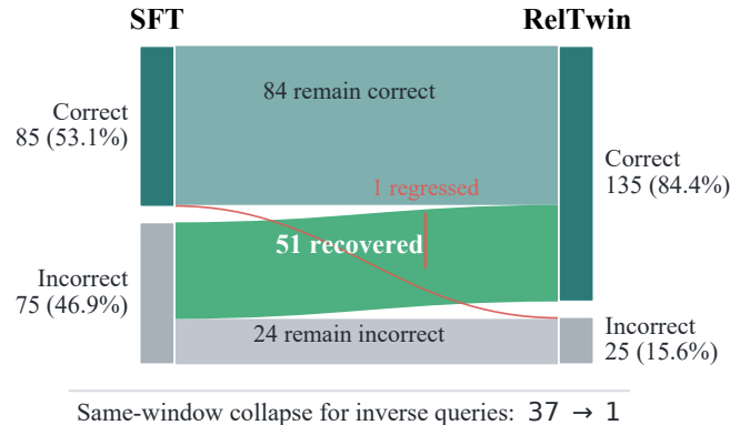
Fig. 2. RelTwin recovers query-window binding failures hidden by aggregate scores. Each ribbon tracks the same inverse-query pair from SFT to RelTwin at the 0.5 joint-IoU threshold ( N = 160 ); 51 pairs are recovered while one regresses. The bottom annotation reports exact same-window predictions for the two inverse queries.
