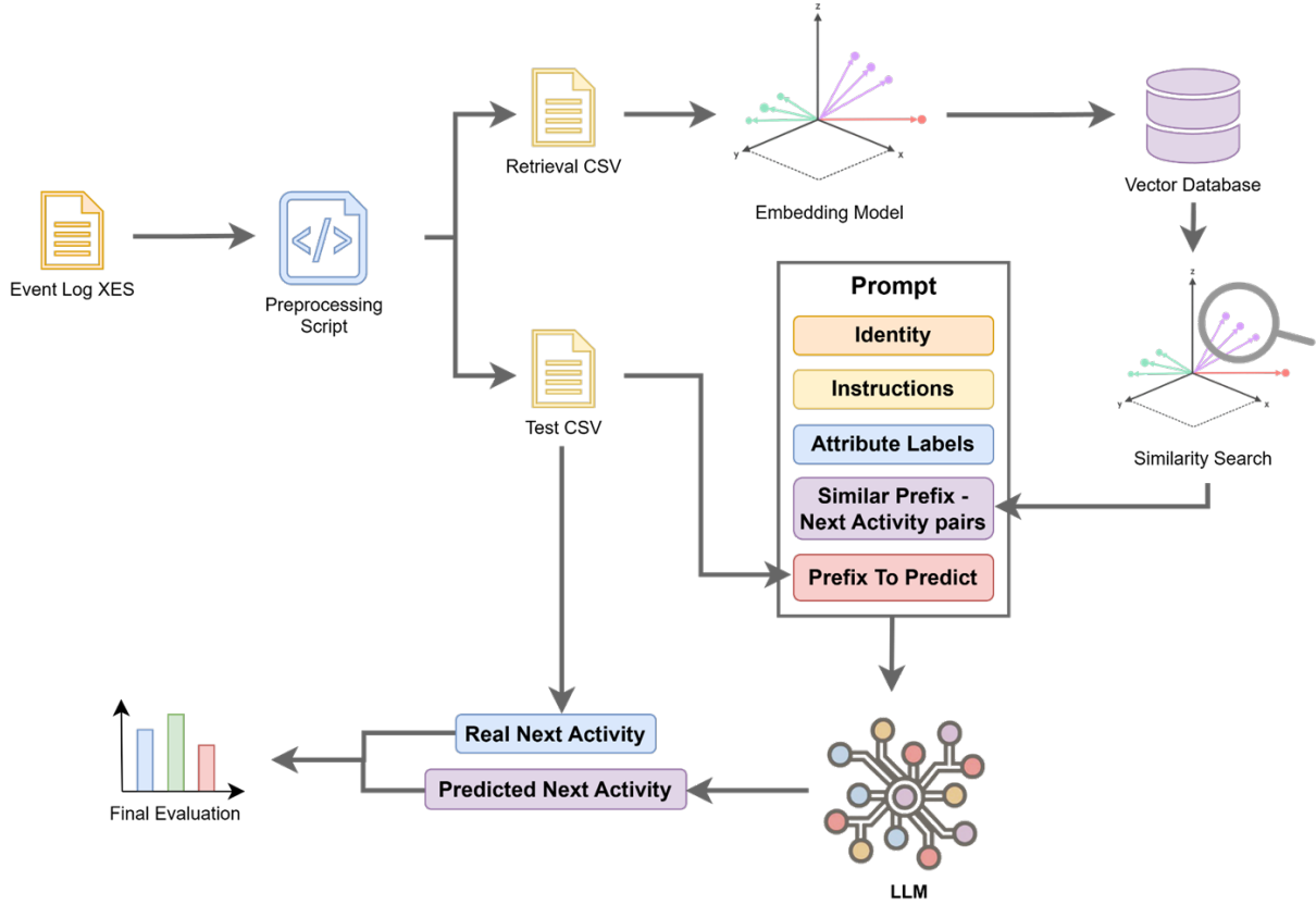
Figure 3.1: High-level overview of the full pipeline and evaluation flow
