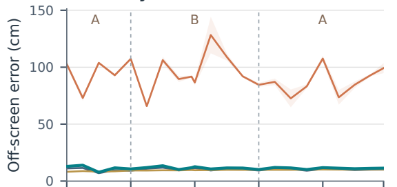
(b) fr1/xyz
