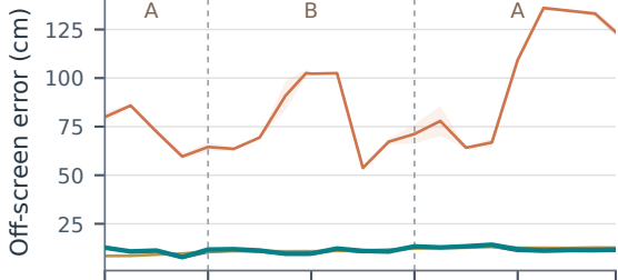
(a) fr1/desk
