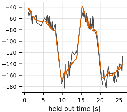
JOINT3: R^2=0.952
