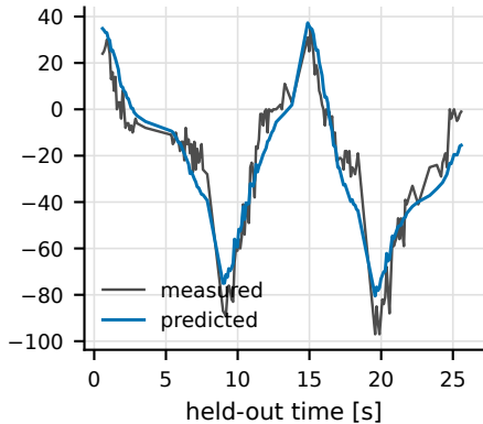
JOINT2: R^2=0.869
