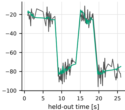
JOINT5: R^2=0.956
