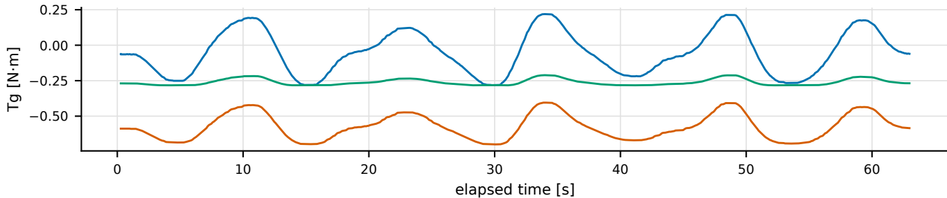
(c) URDF gravity torque
