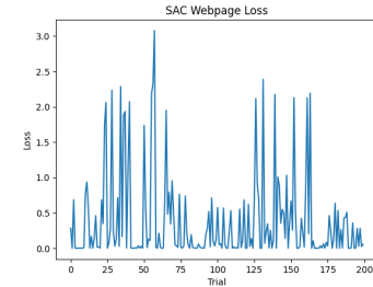
Fig. 3. SAC WP
