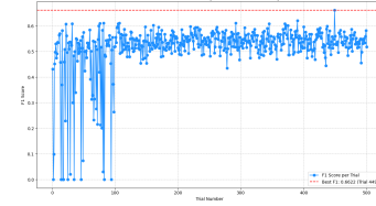
Fig. 2. TD3 WP
