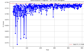
Fig. 5. GPTS WG
