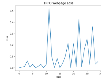
Fig. 4. TRPO WP
