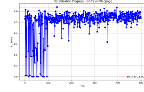
Fig. 1. GPTS WP
