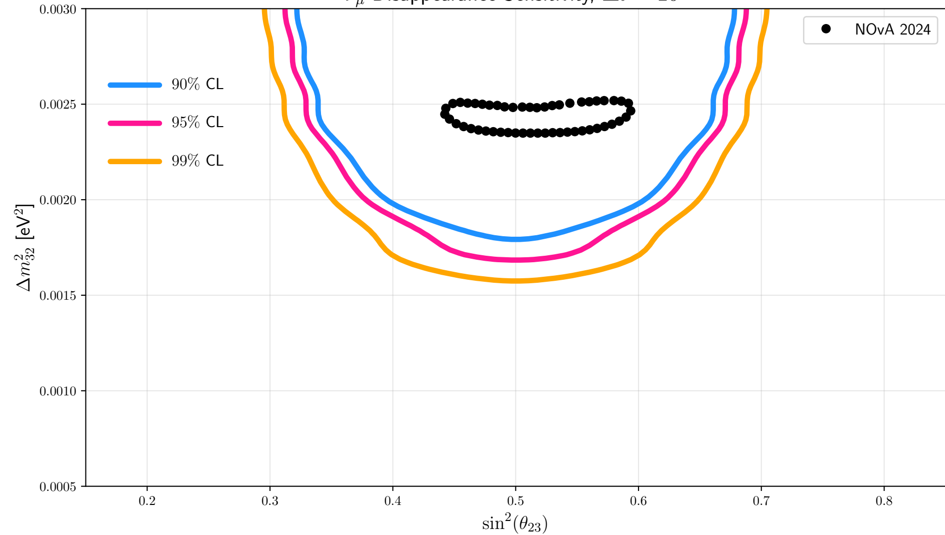
\nu_\mu Disappearance Sensitivity, \Delta\theta = 20^\circ
