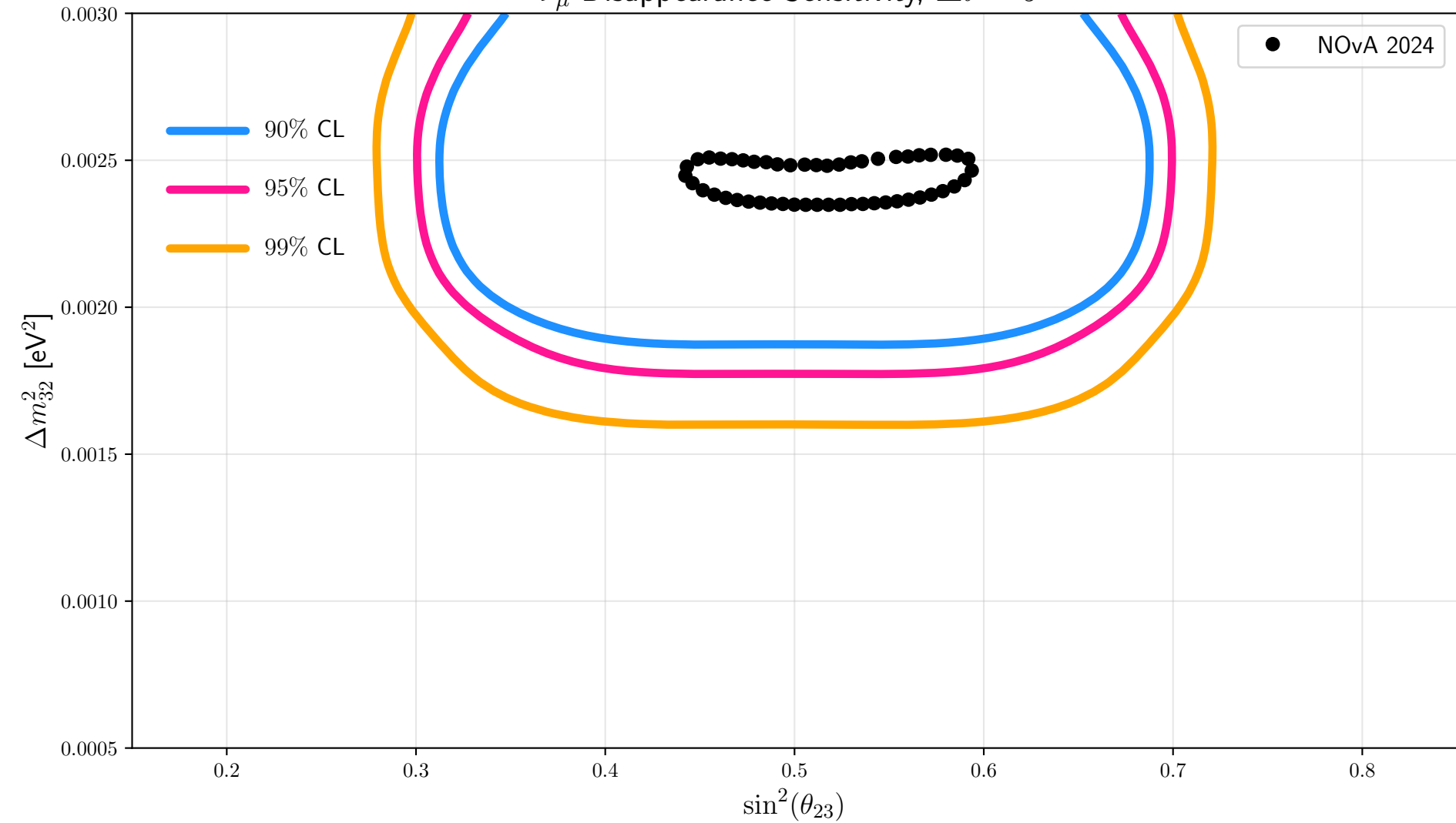
\nu_\mu Disappearance Sensitivity, \Delta\theta = 5^\circ
