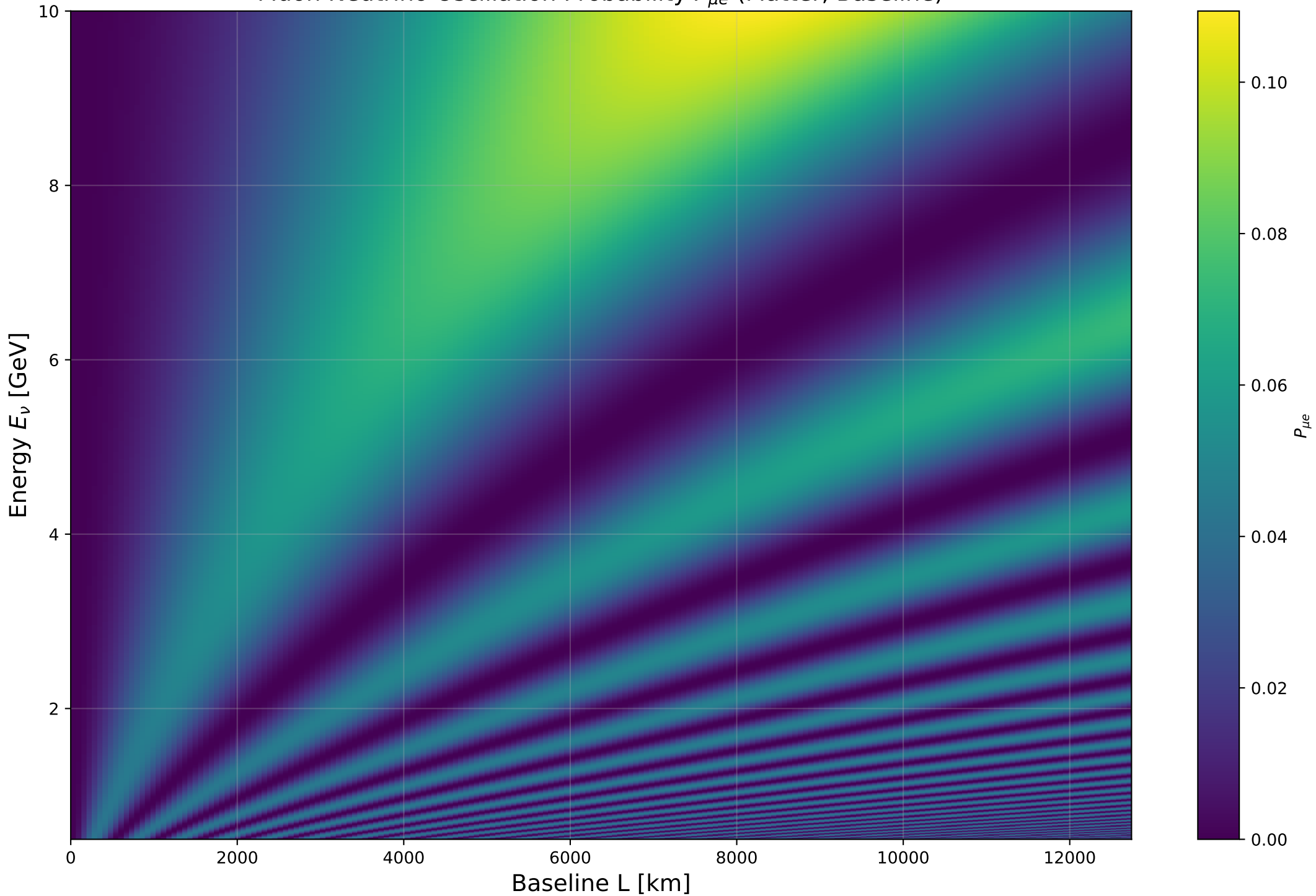
Muon Neutrino Oscillation Probability P_{\mu e} (Matter, Baseline)
