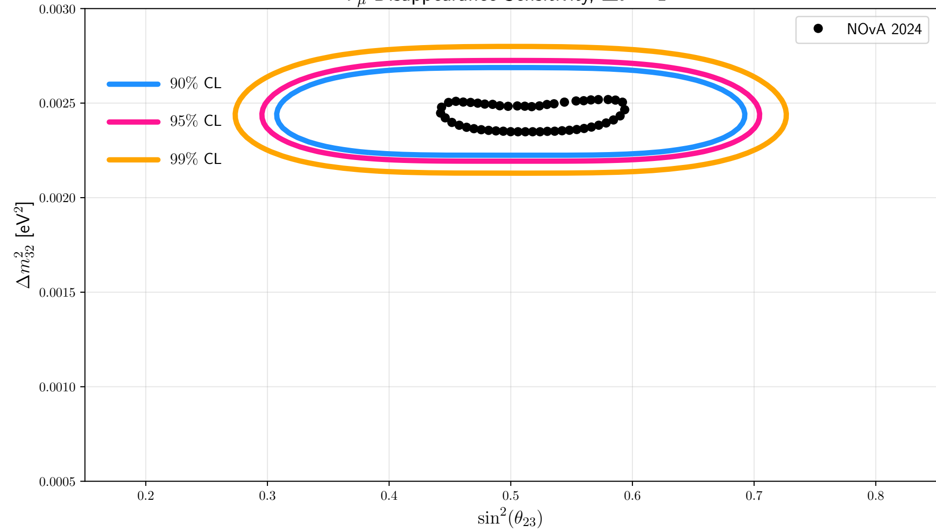
\nu_\mu Disappearance Sensitivity, \Delta\theta = 1^\circ
