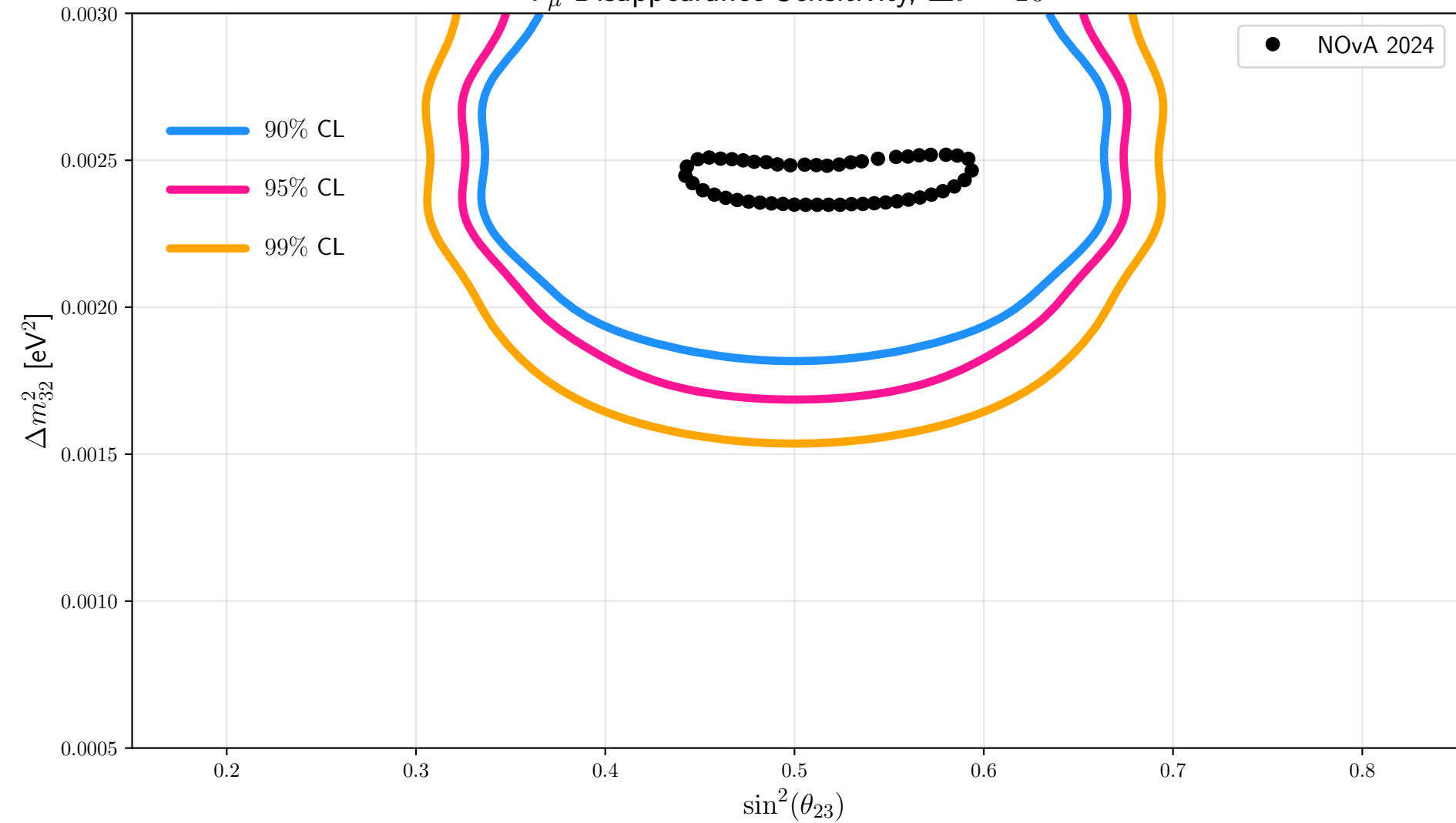
\nu_\mu Disappearance Sensitivity, \Delta\theta = 10^\circ
