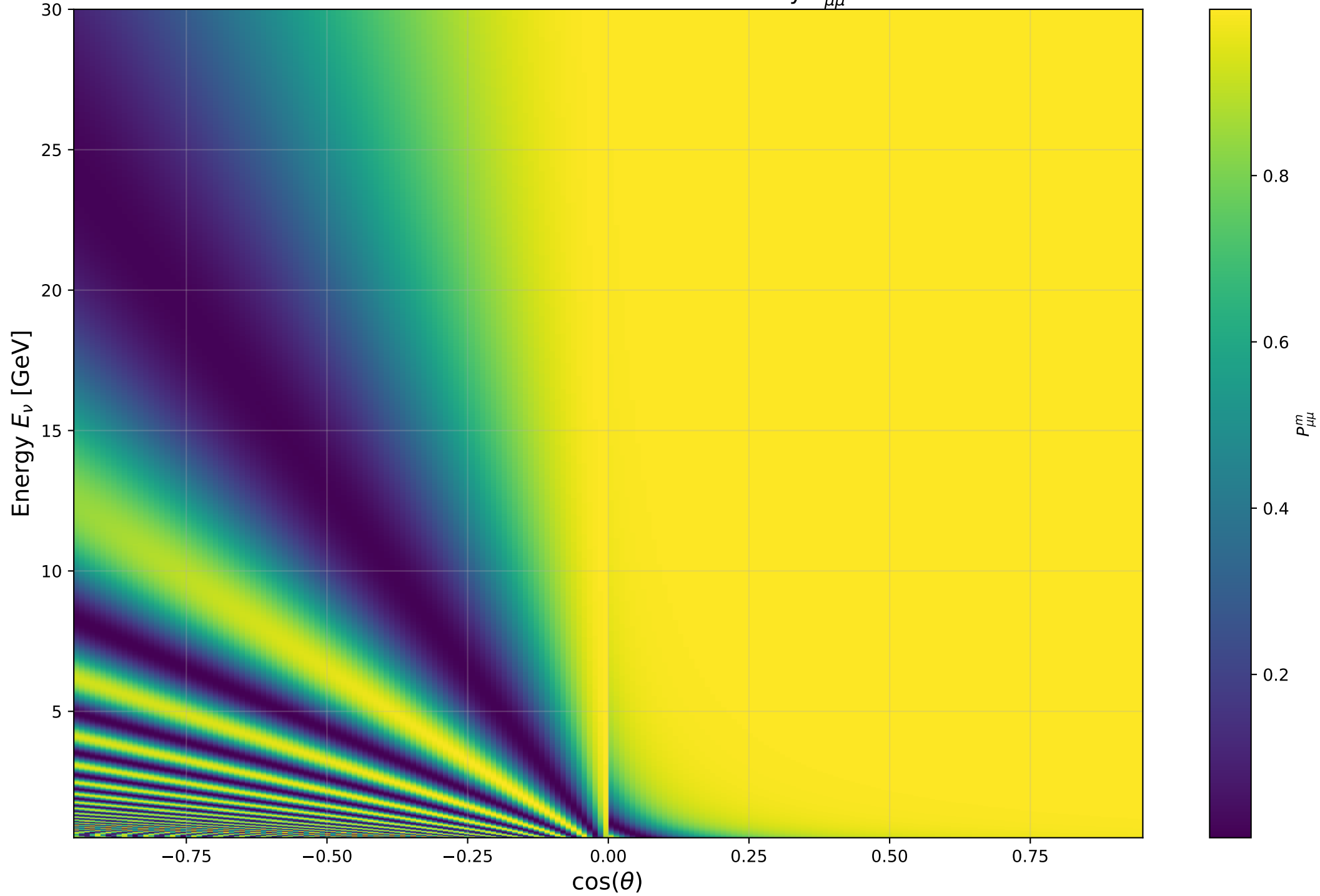
Muon Neutrino Oscillation Probability P_{\mu\mu}^m
