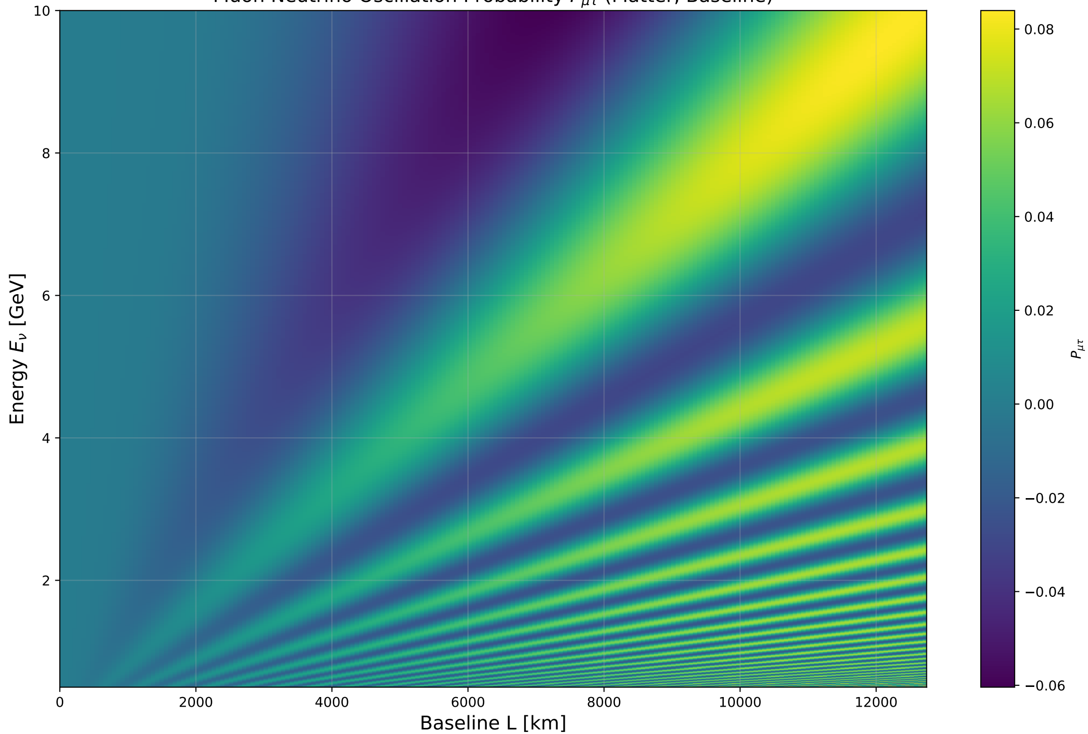
Muon Neutrino Oscillation Probability P_{\mu\tau} (Matter, Baseline)
