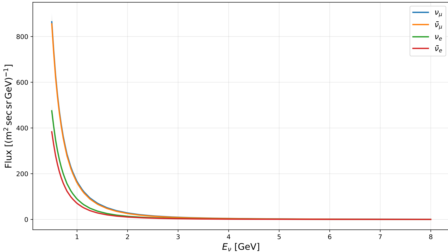
Atmospheric neutrino fluxes at \cos \theta = -0.50
